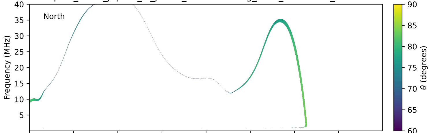
expres_earth_jupiter_io_jrm33_lossc-wid1deg_3kev_19930501_v11.cdf
