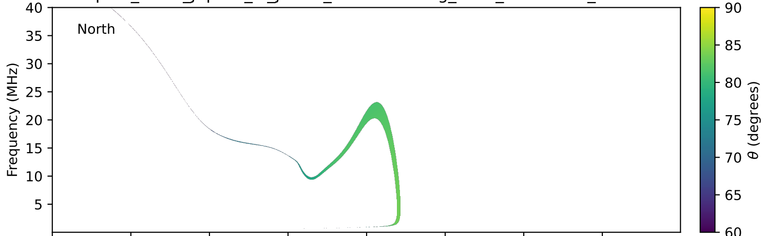
expres_earth_jupiter_io_jrm09_lossc-wid1deg_3kev_19930526_v11.cdf
