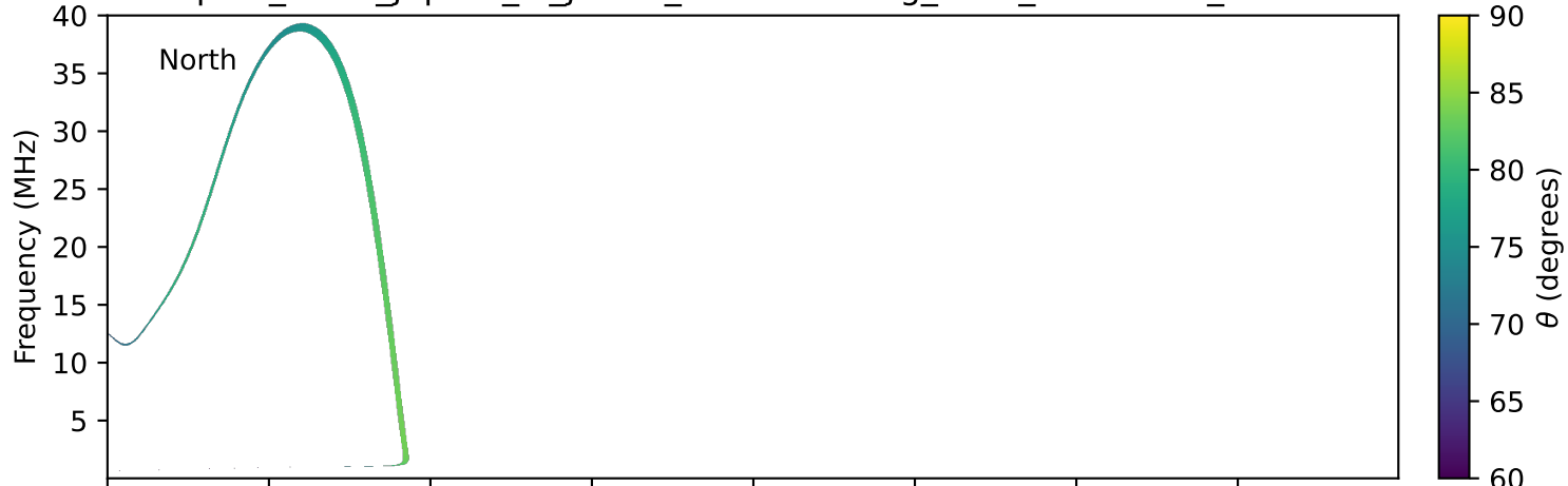
expres_earth_jupiter_io_jrm09_lossc-wid1deg_3kev_19930521_v11.cdf
