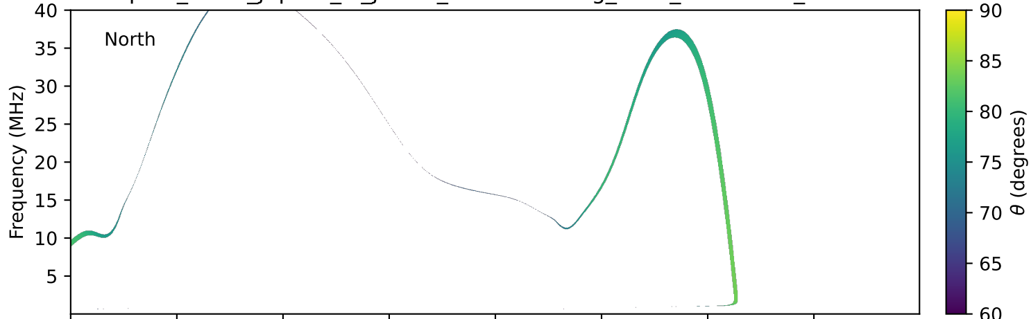
expres_earth_jupiter_io_jrm09_lossc-wid1deg_3kev_19930501_v11.cdf
