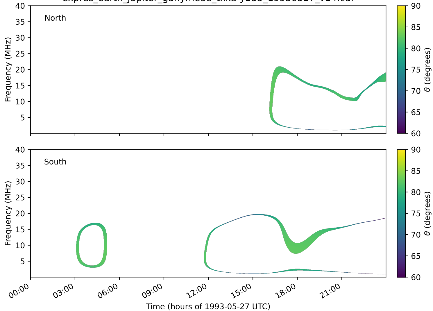
expres_earth_jupiter_ganymede_txka-y235_19930527_v14.cdf
