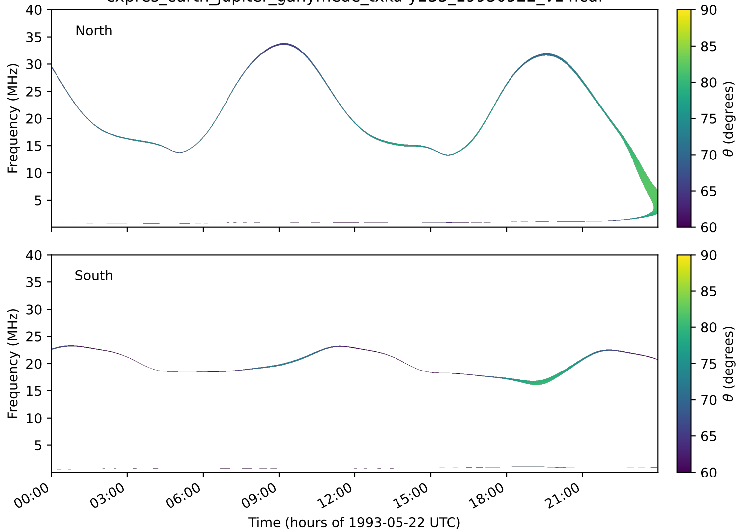
expres_earth_jupiter_ganymede_txka-y235_19930522_v14.cdf
