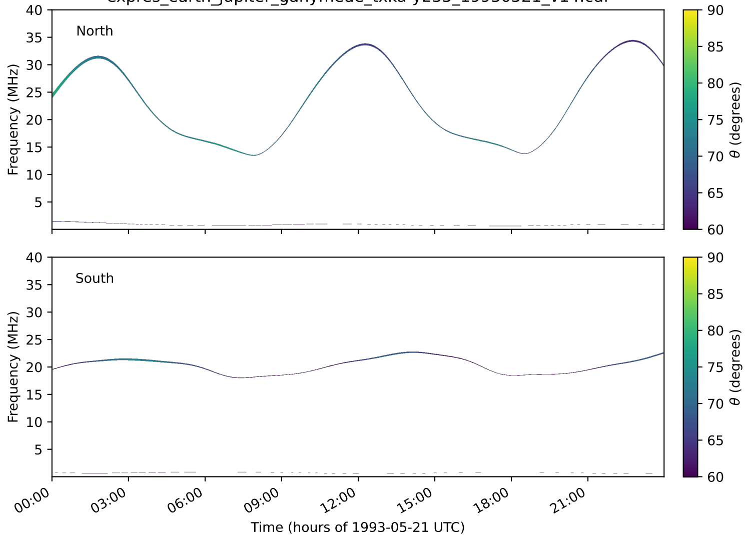
expres_earth_jupiter_ganymede_txka-y235_19930521_v14.cdf
