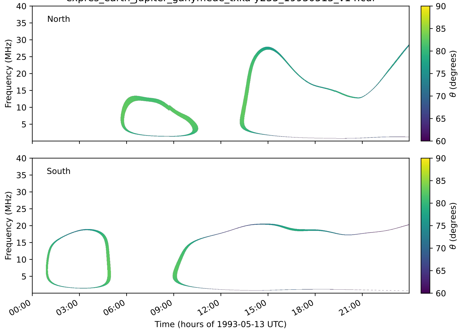
expres_earth_jupiter_ganymede_txka-y235_19930513_v14.cdf
