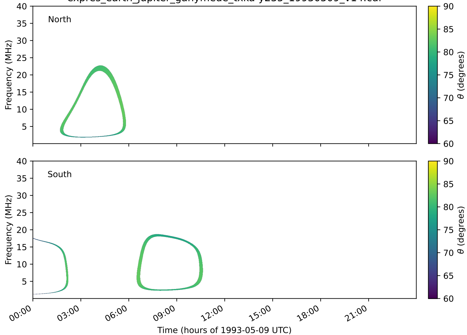
expres_earth_jupiter_ganymede_txka-y235_19930509_v14.cdf
