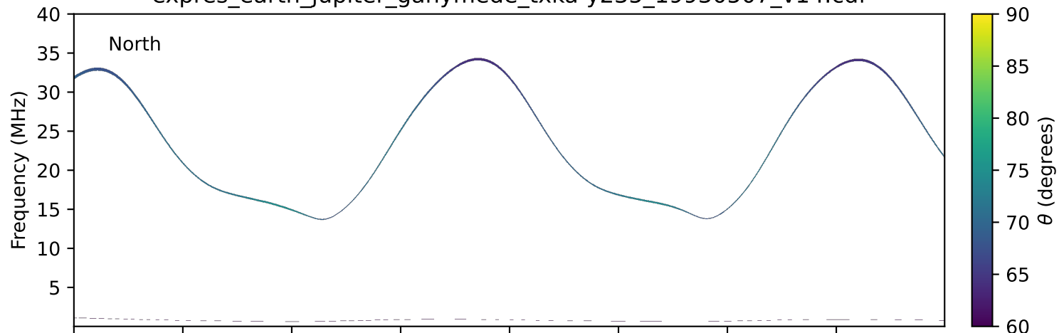
expres_earth_jupiter_ganymede_txka-y235_19930507_v14.cdf
