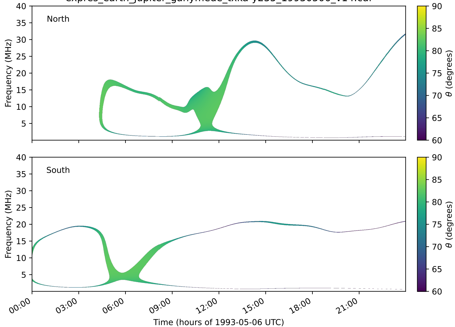
expres_earth_jupiter_ganymede_txka-y235_19930506_v14.cdf
