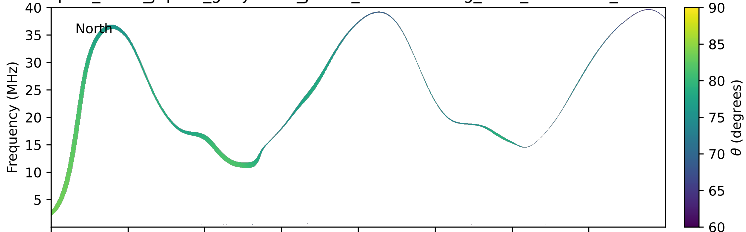
expres_earth_jupiter_ganymede_jrm33_lossc-wid1deg_3kev_19930528_v11.cdf
