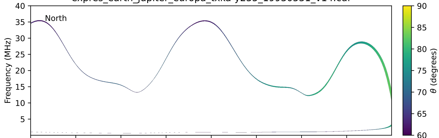
expres_earth_jupiter_europa_txka-y235_19930531_v14.cdf
