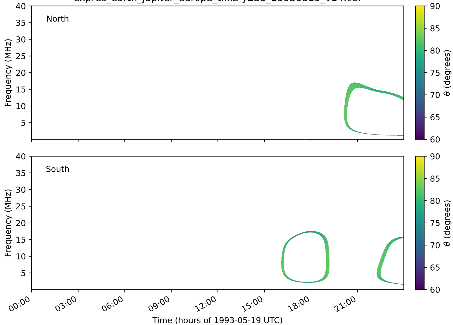
expres_earth_jupiter_europa_txka-y235_19930519_v14.cdf
