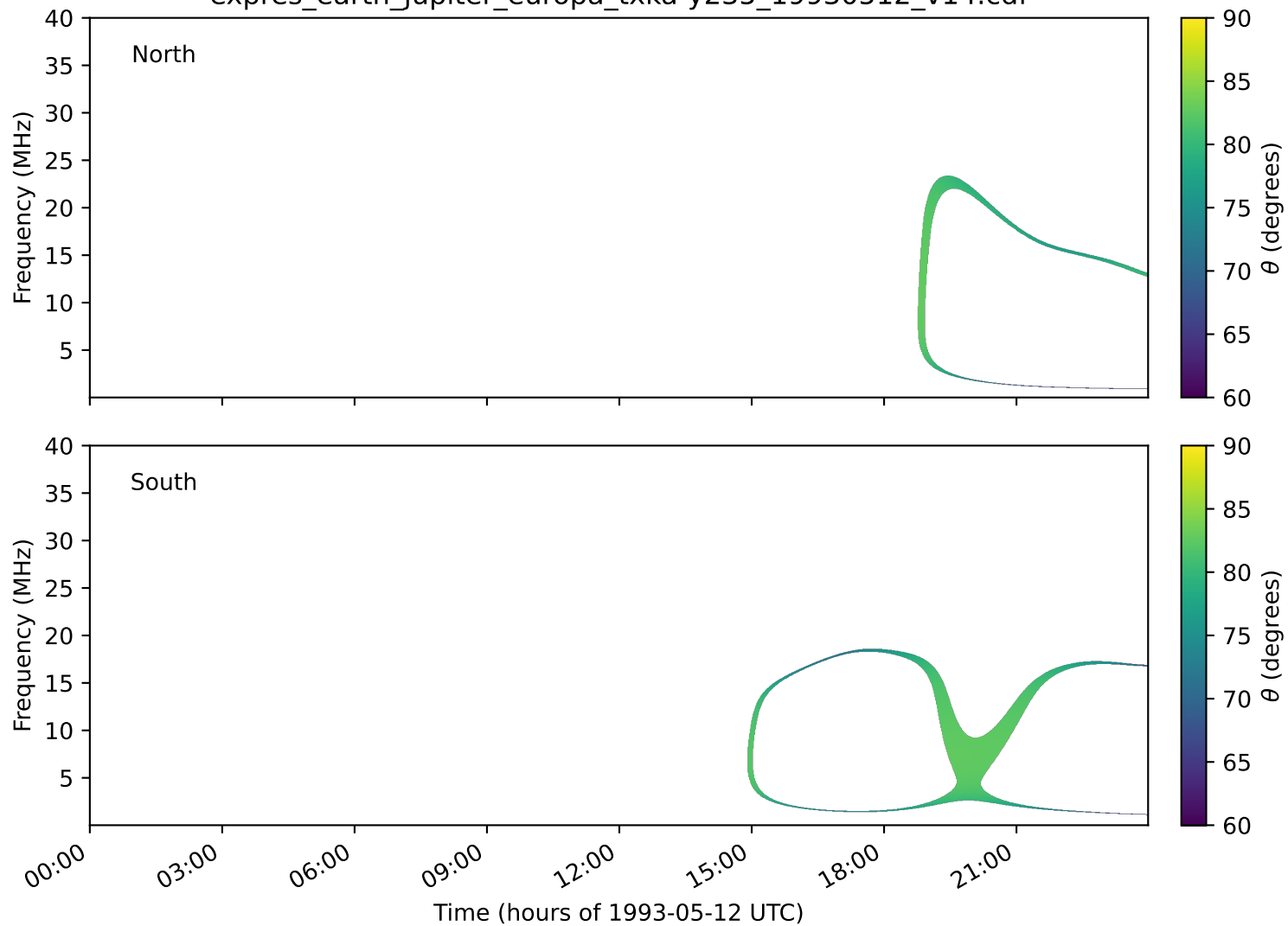
expres_earth_jupiter_europa_txka-y235_19930512_v14.cdf
