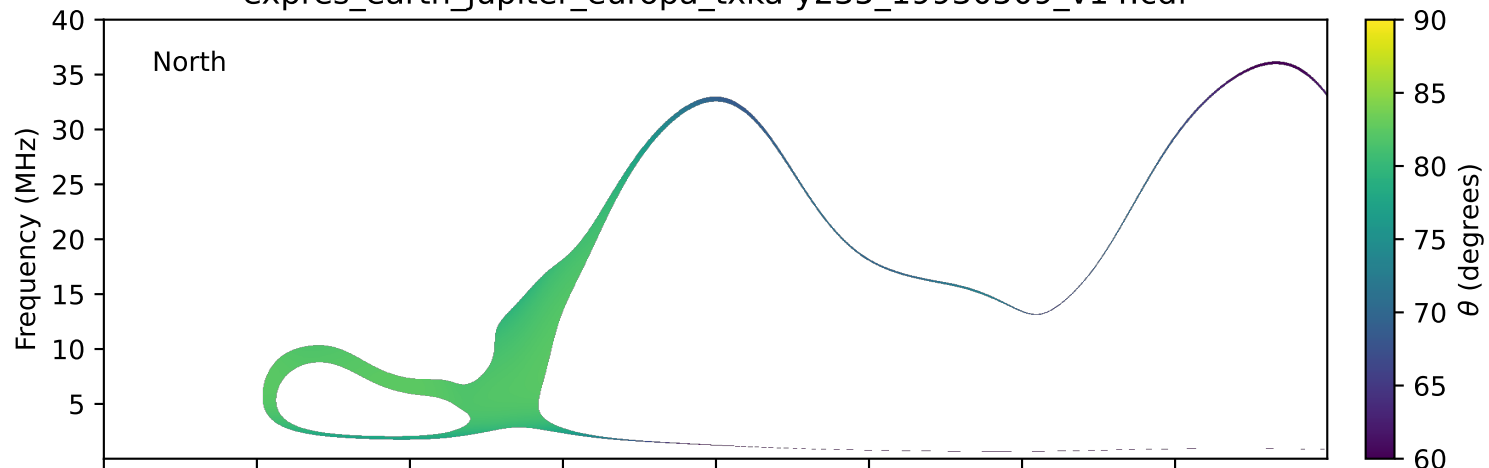
expres_earth_jupiter_europa_txka-y235_19930509_v14.cdf
