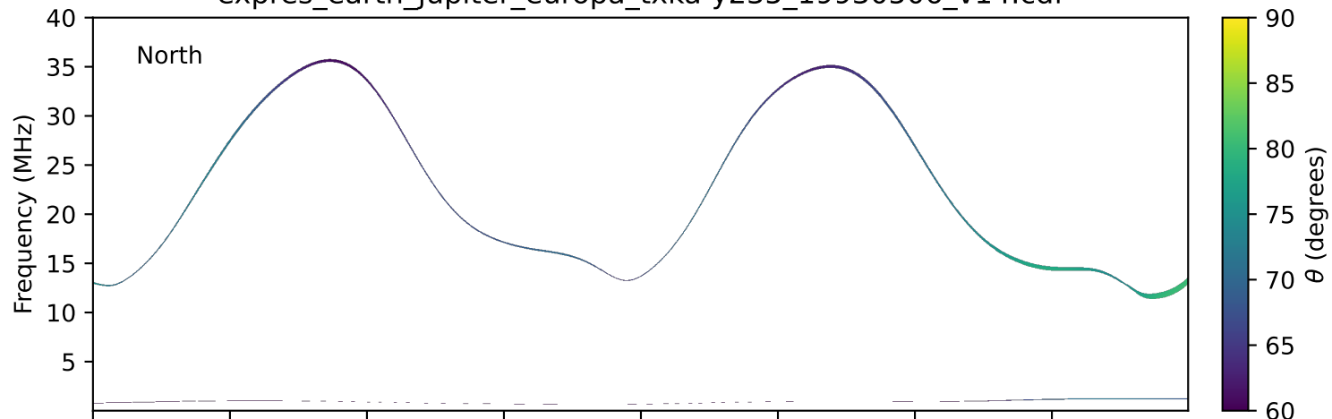
expres_earth_jupiter_europa_txka-y235_19930506_v14.cdf
