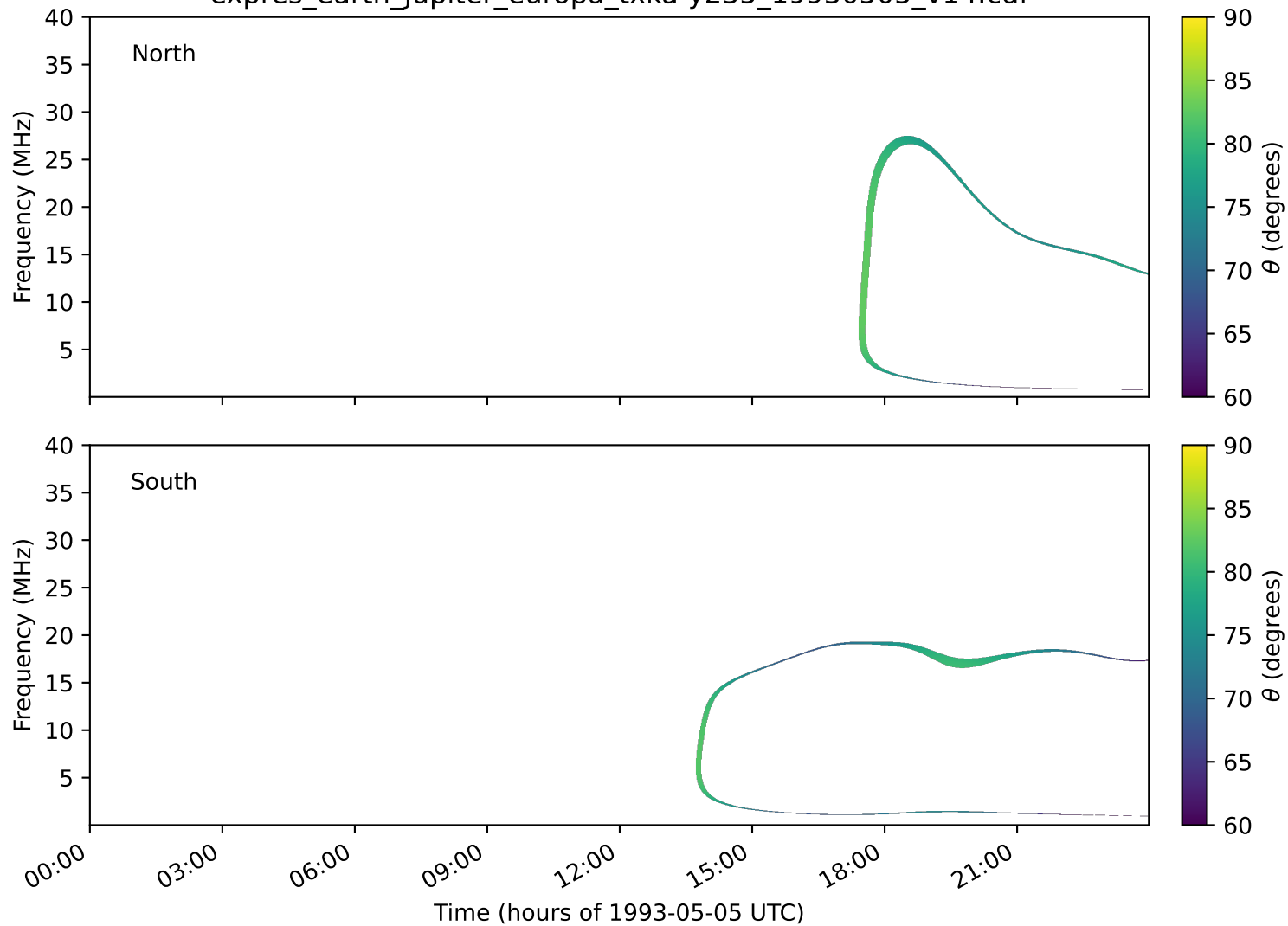
expres_earth_jupiter_europa_txka-y235_19930505_v14.cdf
