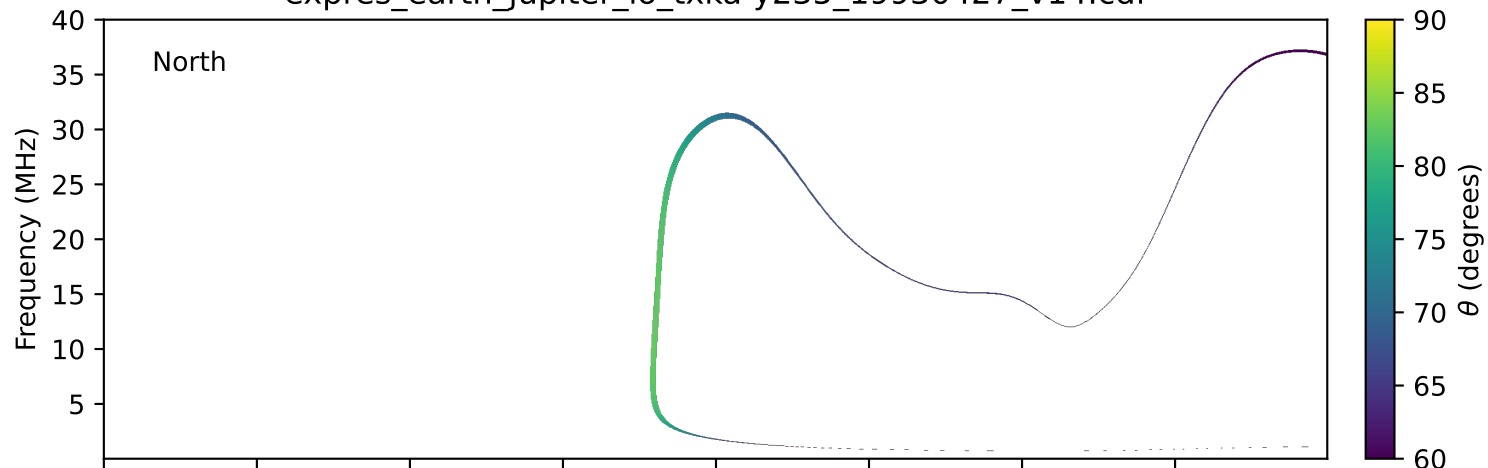
expres_earth_jupiter_io_txka-y235_19930427_v14.cdf
