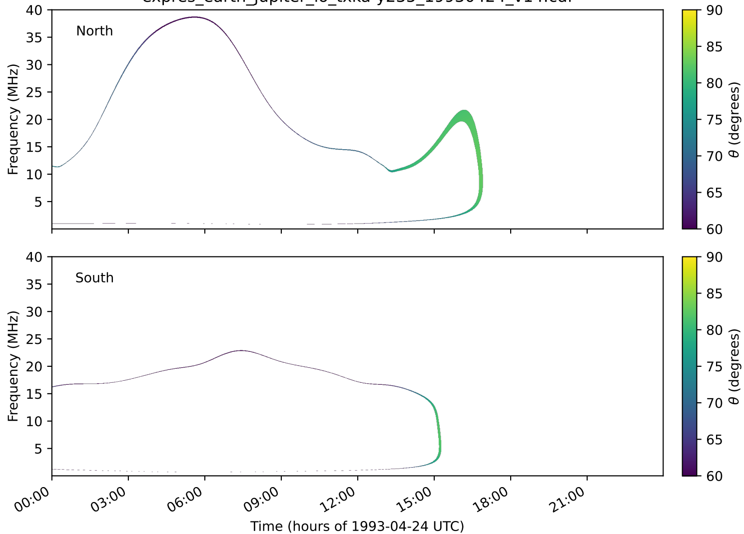
expres_earth_jupiter_io_txka-y235_19930424_v14.cdf
