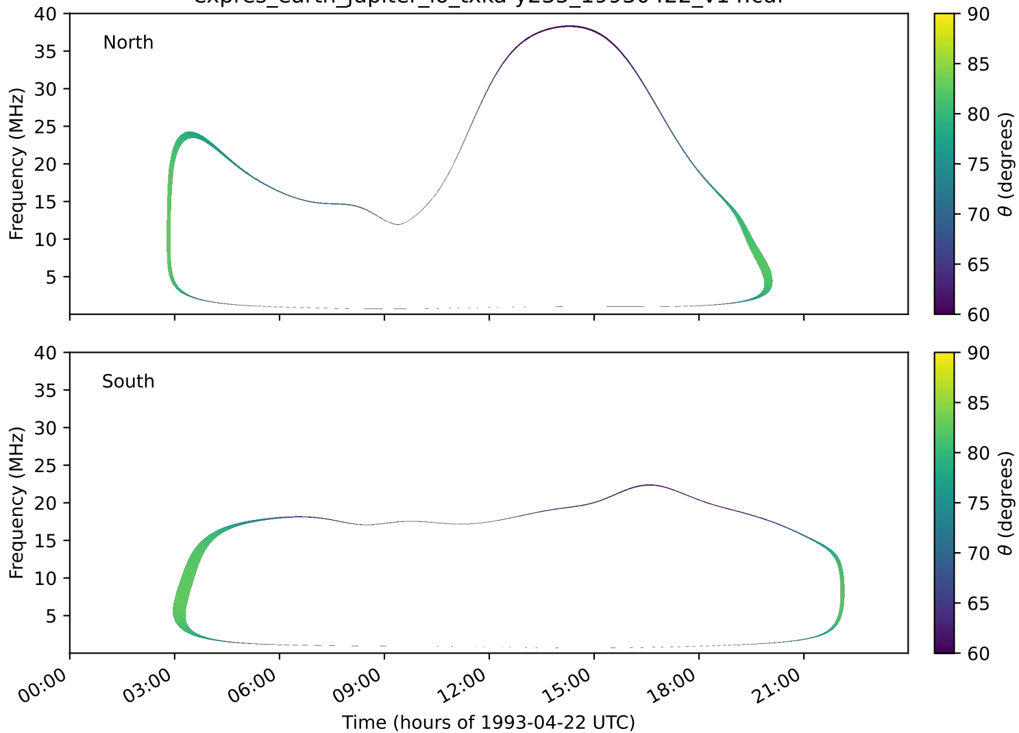
expres_earth_jupiter_io_txka-y235_19930422_v14.cdf
