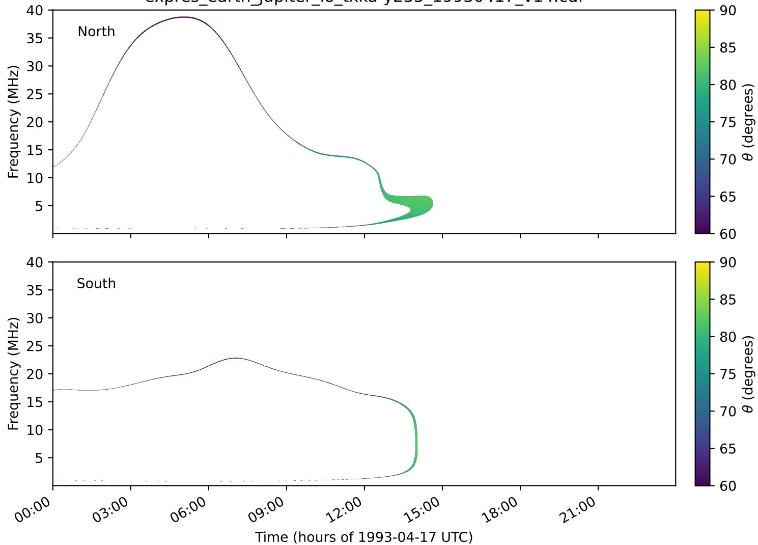
expres_earth_jupiter_io_txka-y235_19930417_v14.cdf
