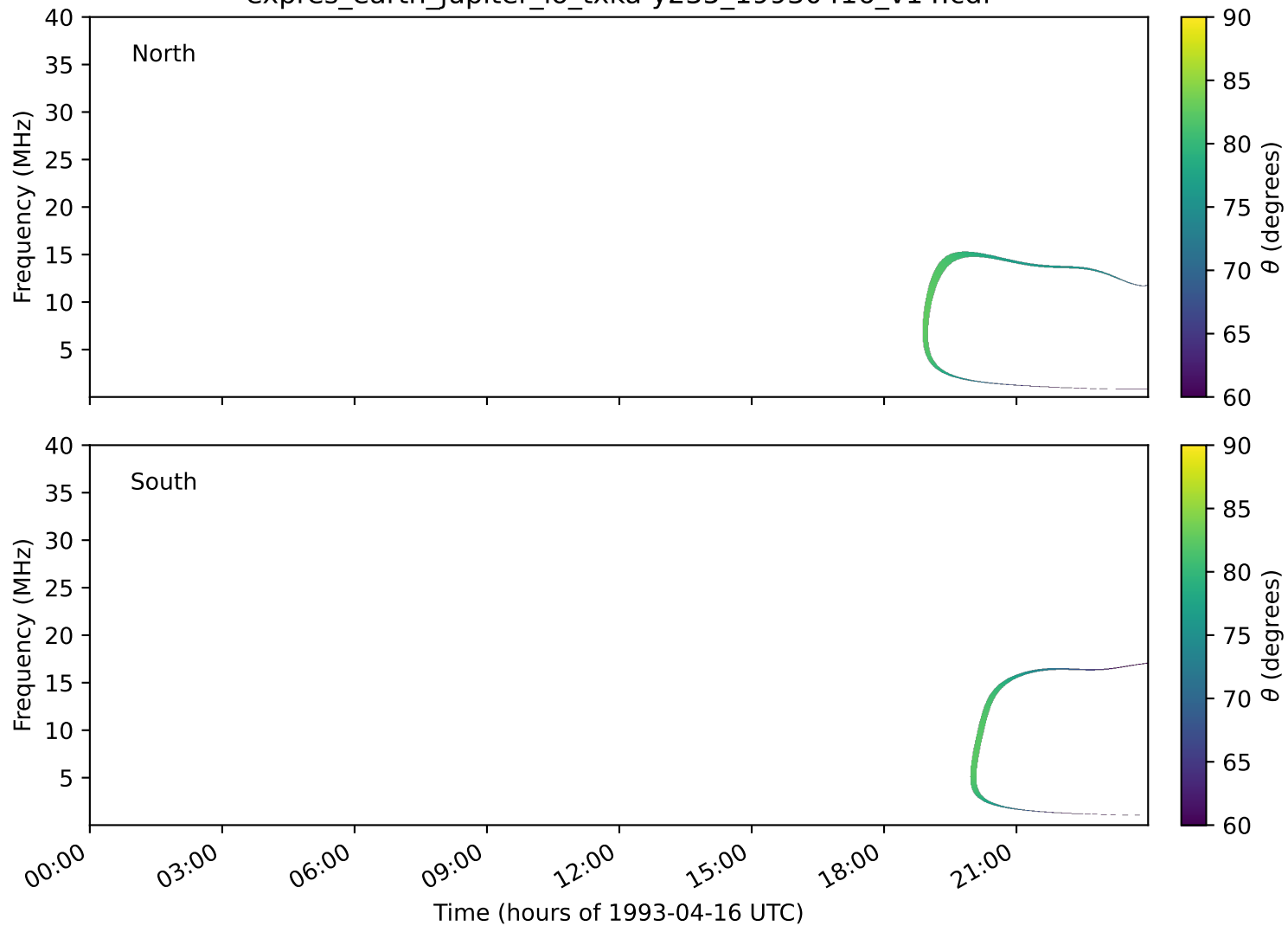
expres_earth_jupiter_io_txka-y235_19930416_v14.cdf
