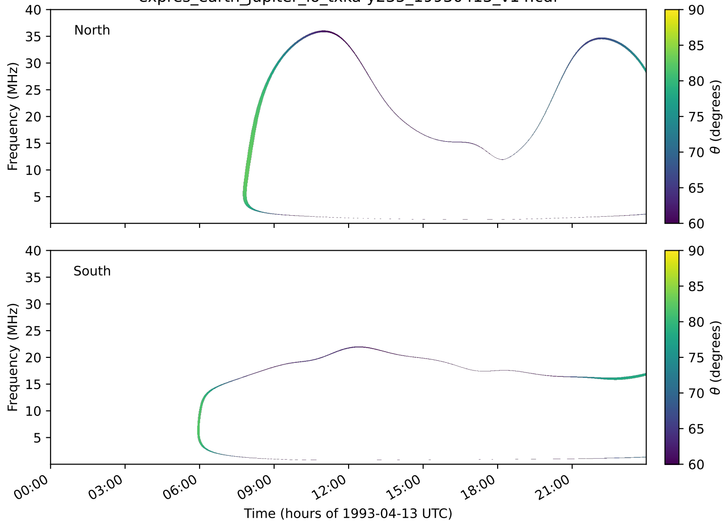
expres_earth_jupiter_io_txka-y235_19930413_v14.cdf
