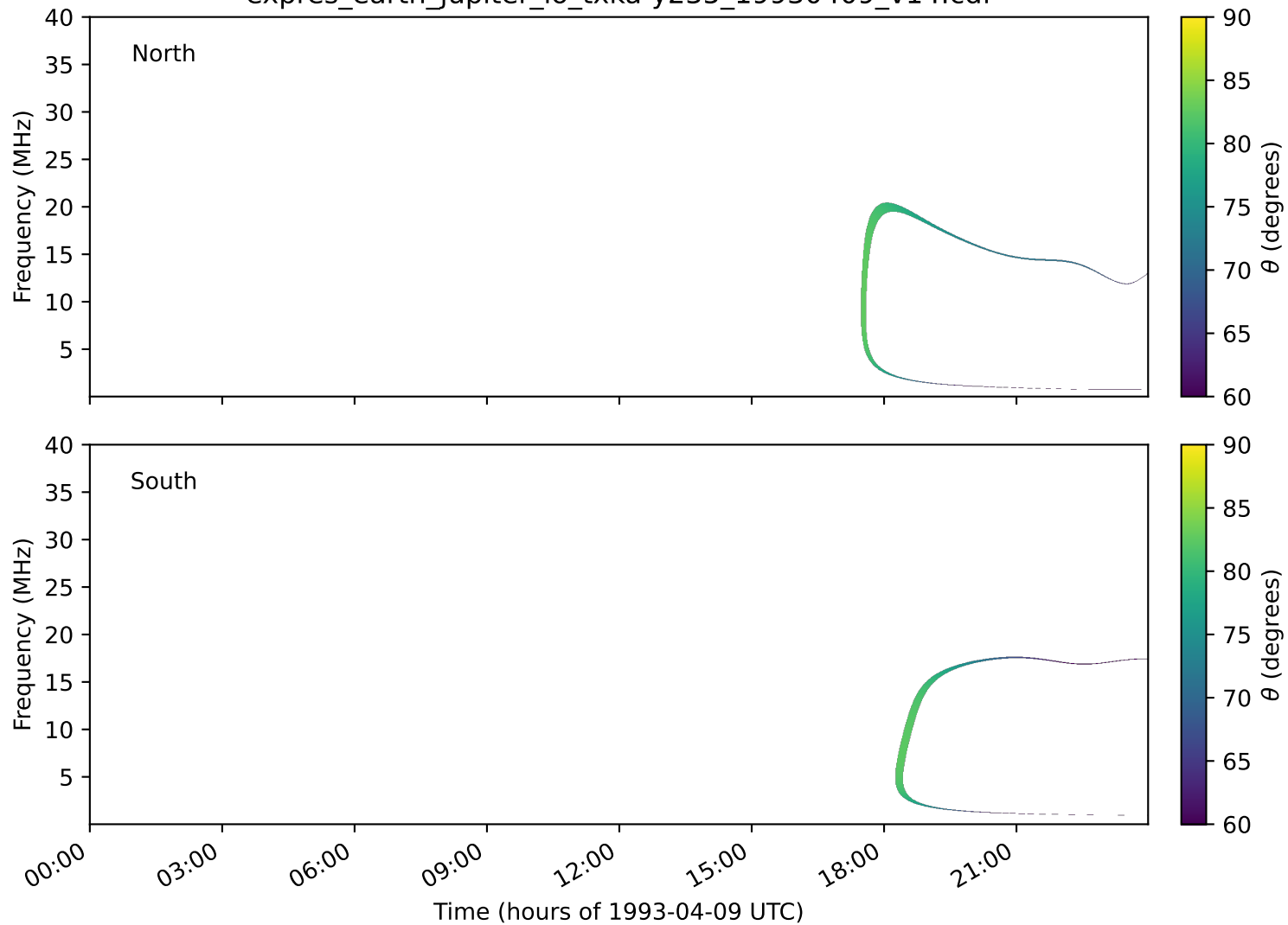
expres_earth_jupiter_io_txka-y235_19930409_v14.cdf
