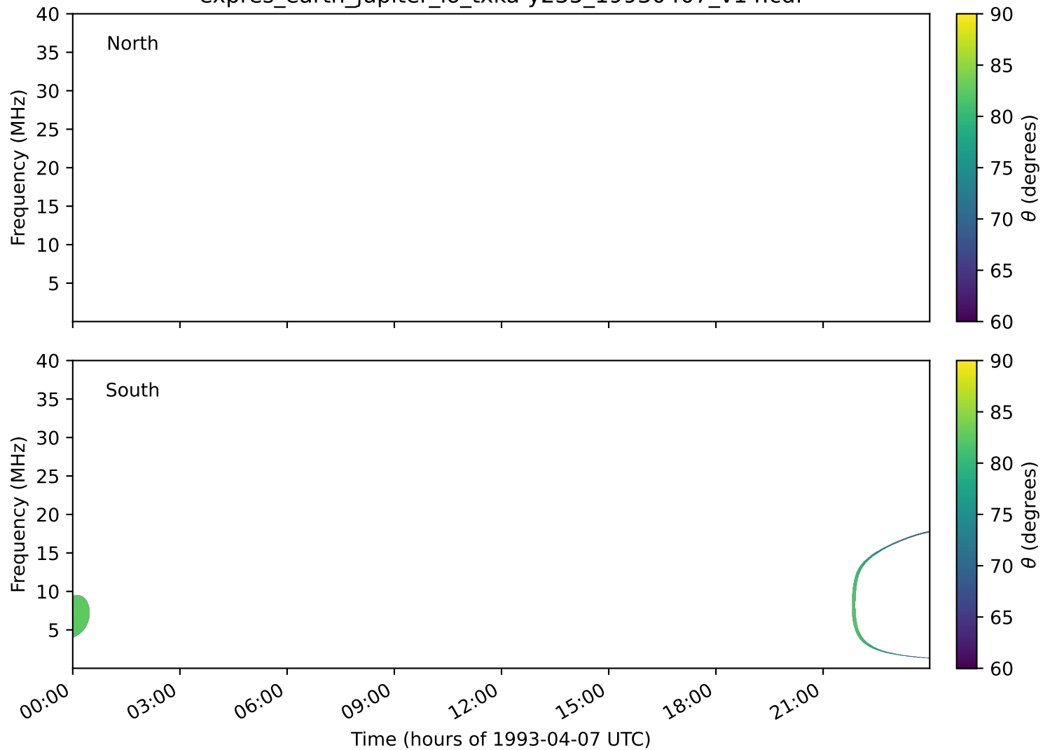
expres_earth_jupiter_io_txka-y235_19930407_v14.cdf
