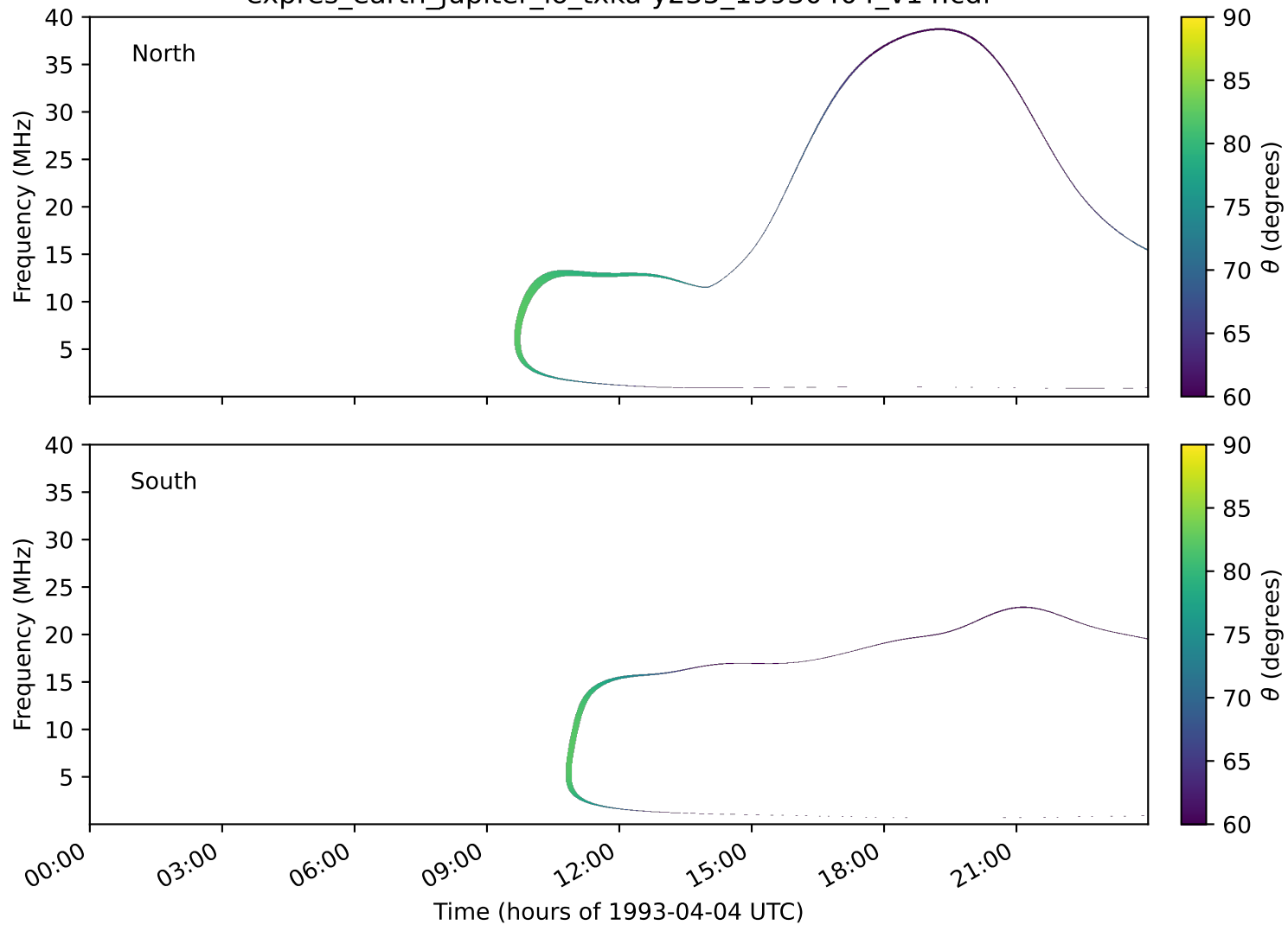
expres_earth_jupiter_io_txka-y235_19930404_v14.cdf
