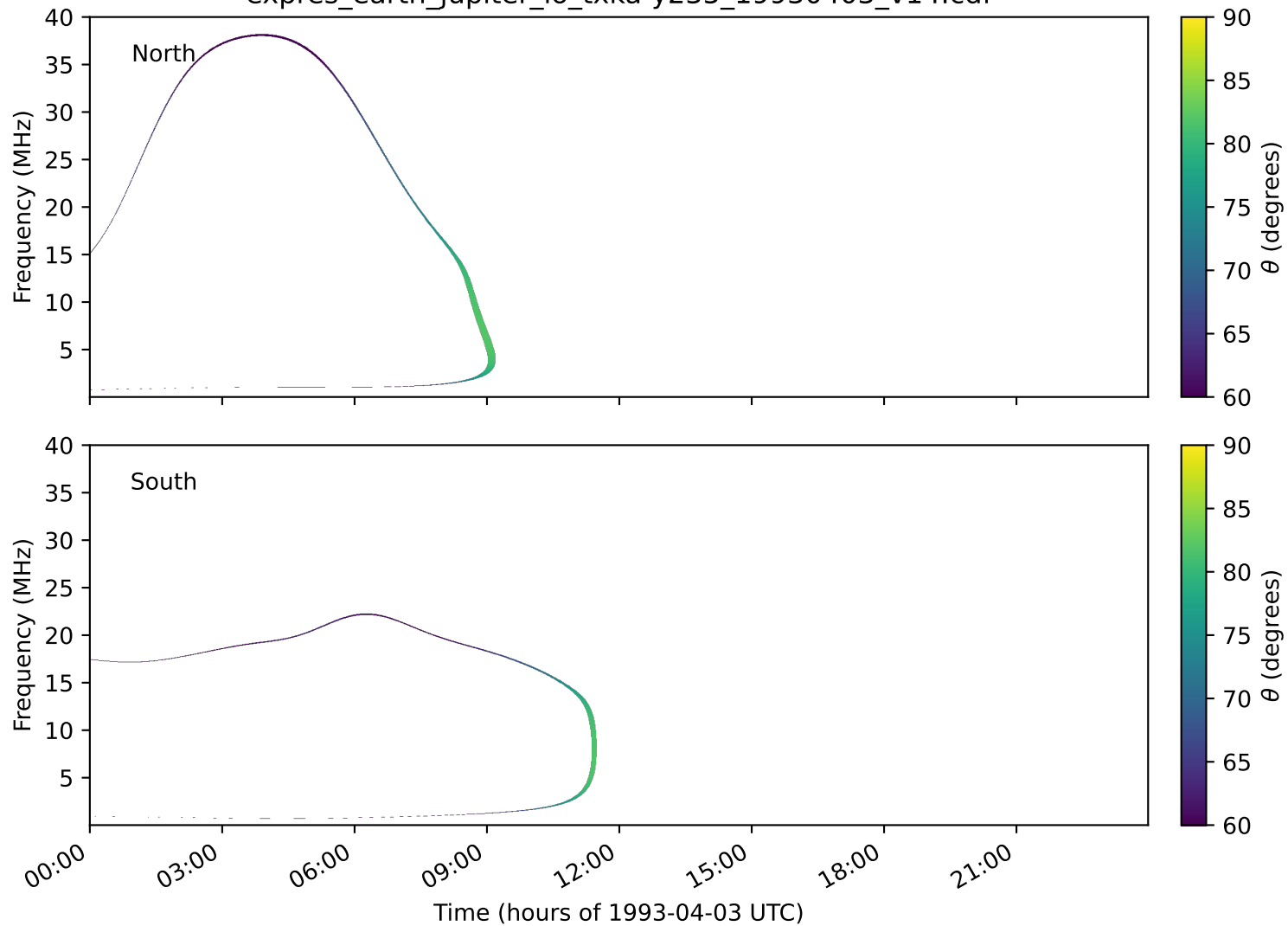
expres_earth_jupiter_io_txka-y235_19930403_v14.cdf
