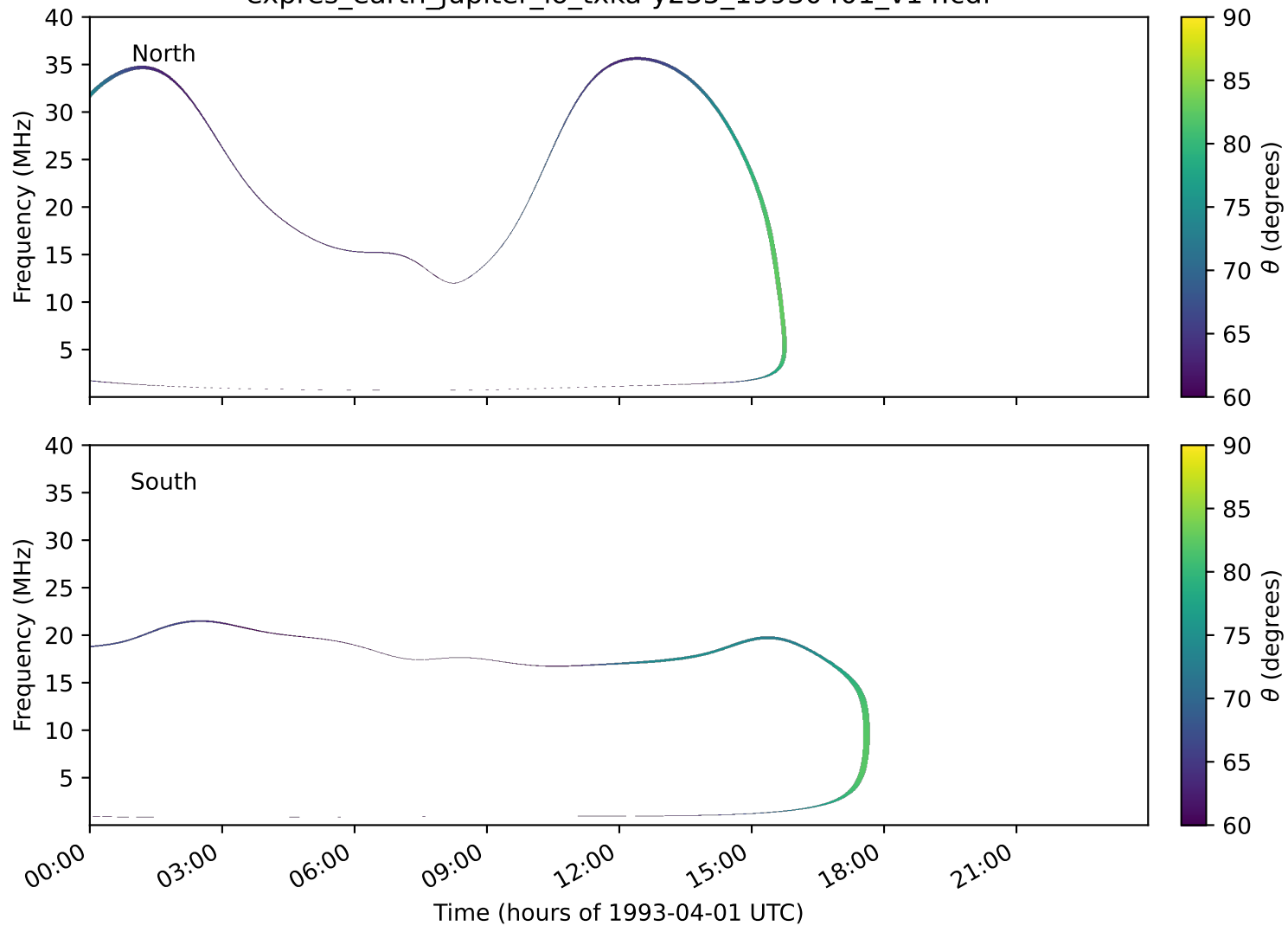
expres_earth_jupiter_io_txka-y235_19930401_v14.cdf
