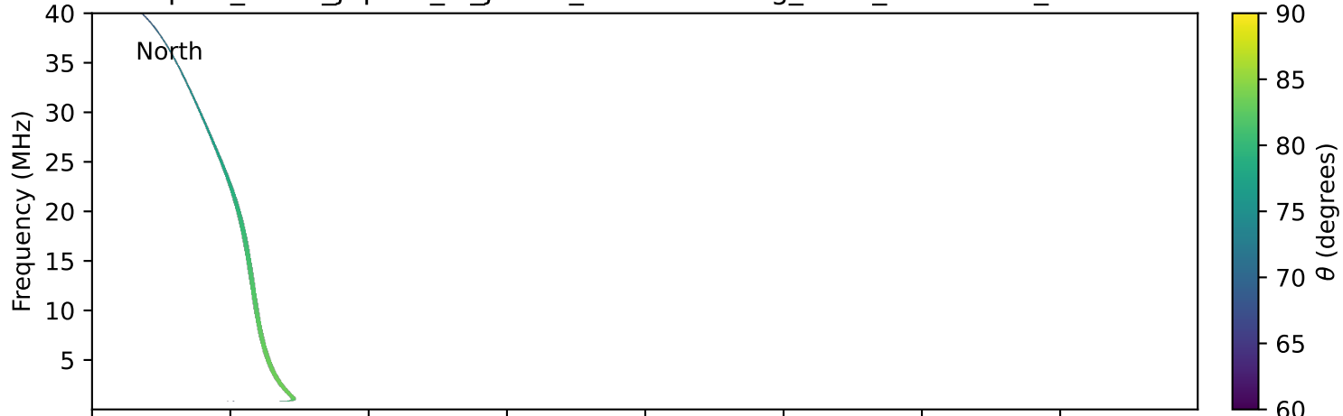
expres_earth_jupiter_io_jrm33_lossc-wid1deg_3kev_19930428_v11.cdf
