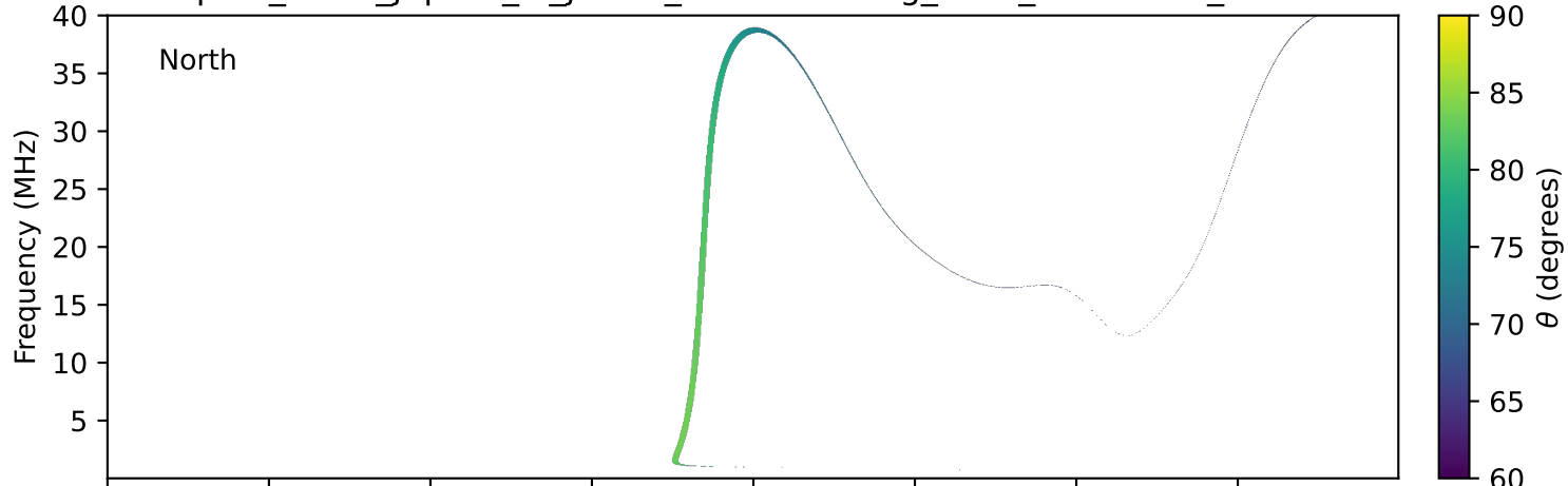
expres_earth_jupiter_io_jrm33_lossc-wid1deg_3kev_19930427_v11.cdf
