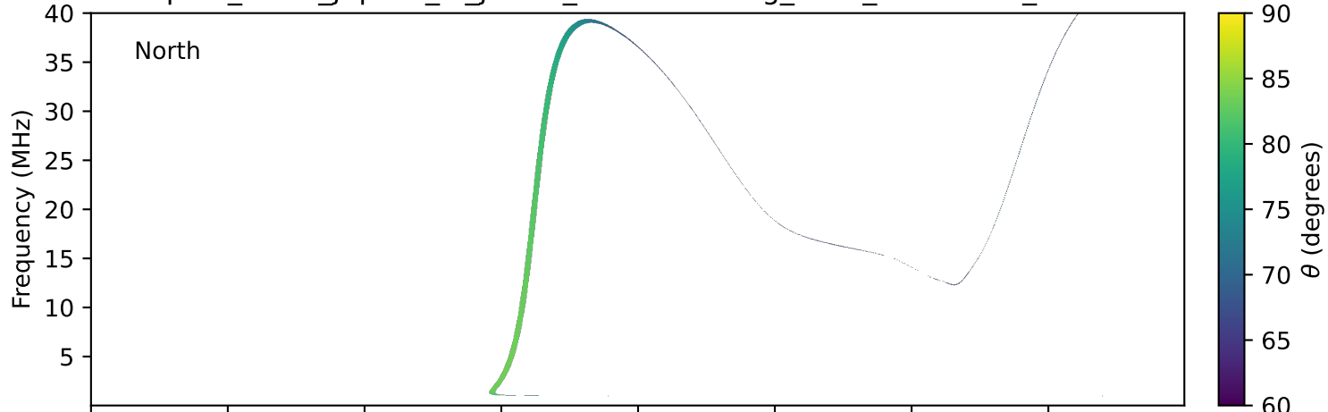
expres_earth_jupiter_io_jrm09_lossc-wid1deg_3kev_19930420_v11.cdf
