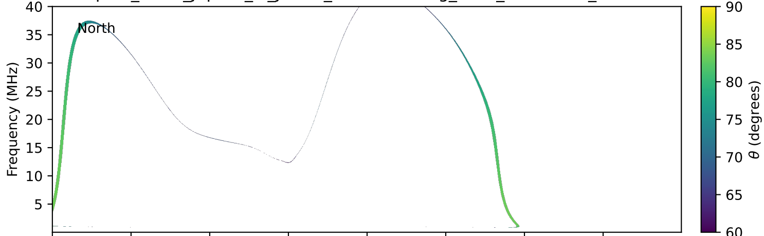
expres_earth_jupiter_io_jrm09_lossc-wid1deg_3kev_19930408_v11.cdf
