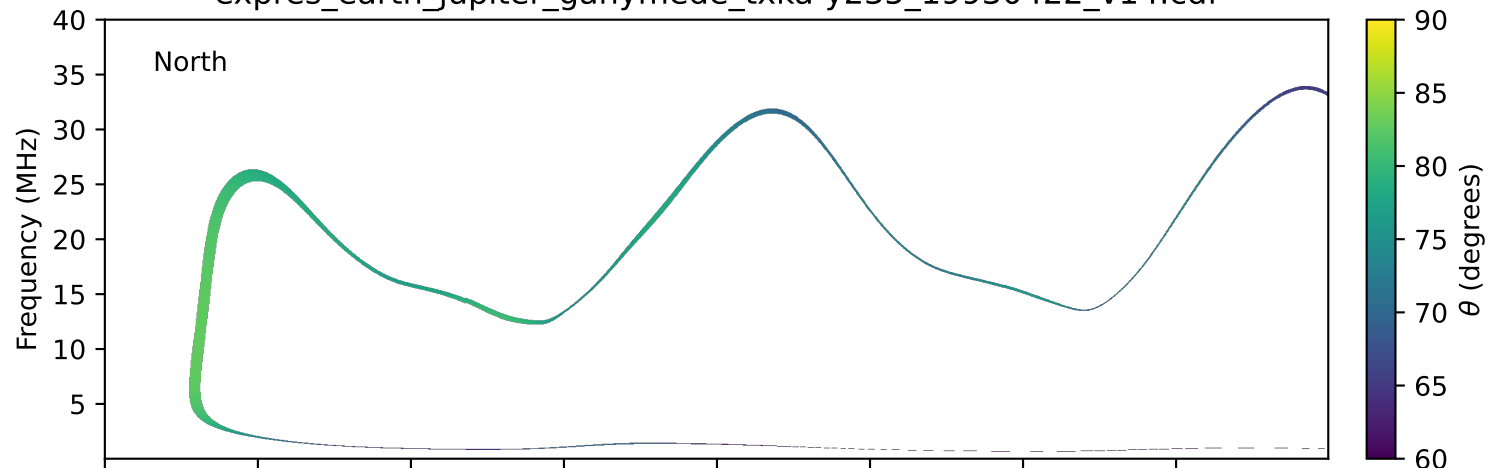
expres_earth_jupiter_ganymede_txka-y235_19930422_v14.cdf
