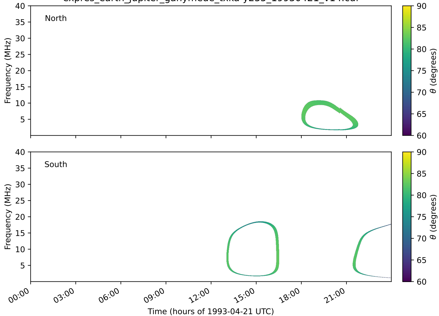
expres_earth_jupiter_ganymede_txka-y235_19930421_v14.cdf
