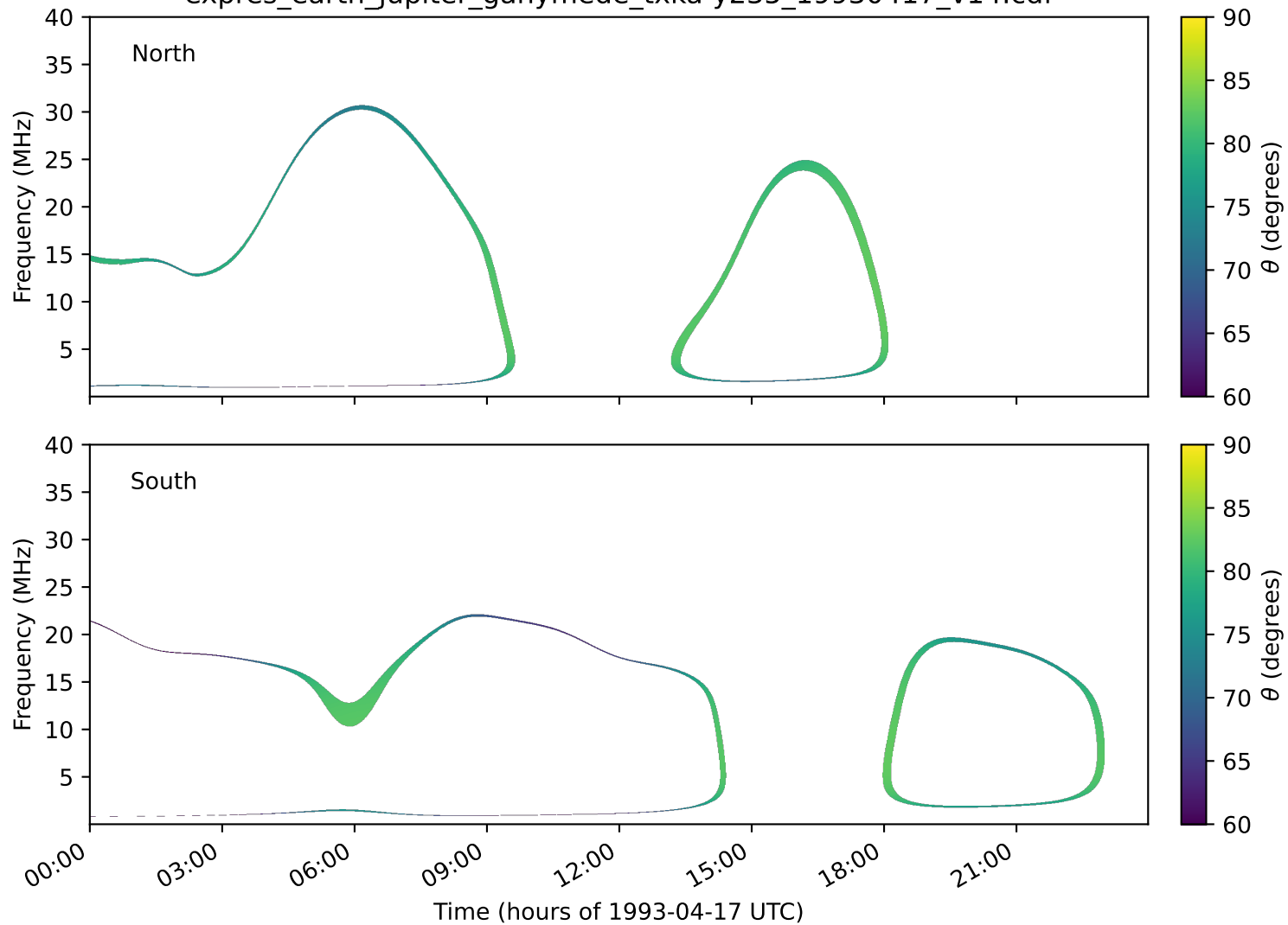
expres_earth_jupiter_ganymede_txka-y235_19930417_v14.cdf
