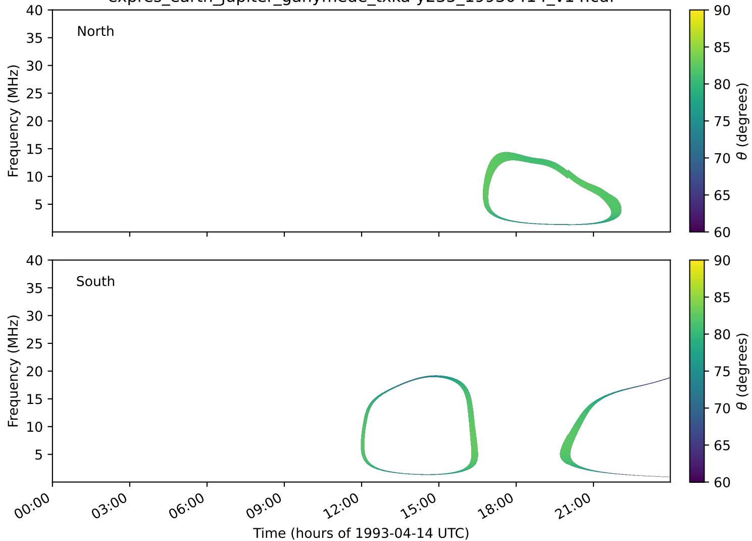
expres_earth_jupiter_ganymede_txka-y235_19930414_v14.cdf
