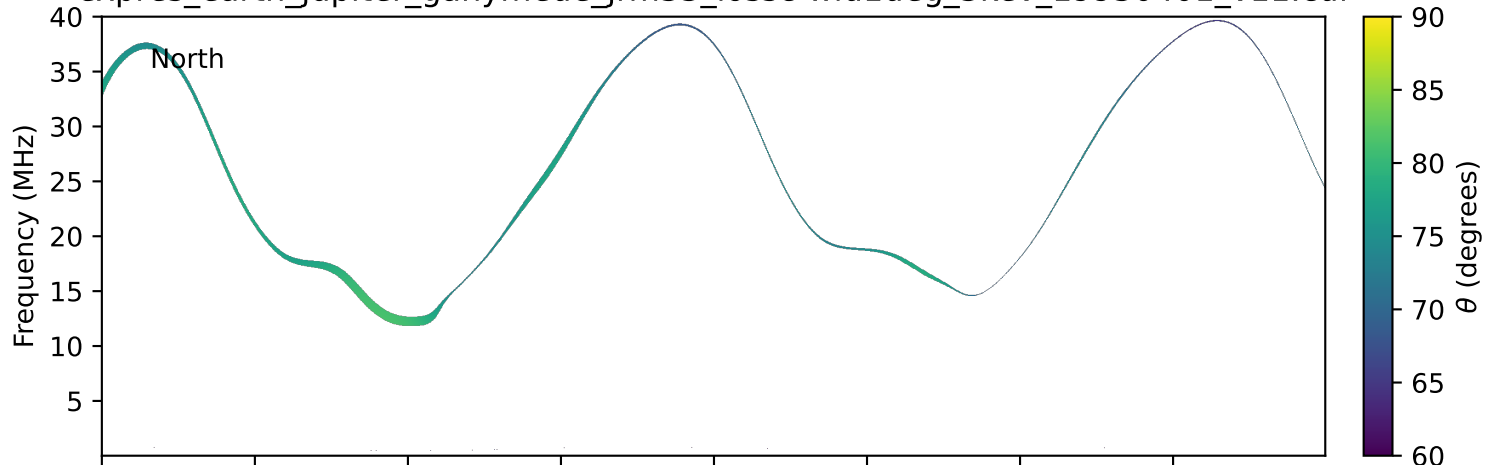
expres_earth_jupiter_ganymede_jrm33_lossc-wid1deg_3kev_19930401_v11.cdf
