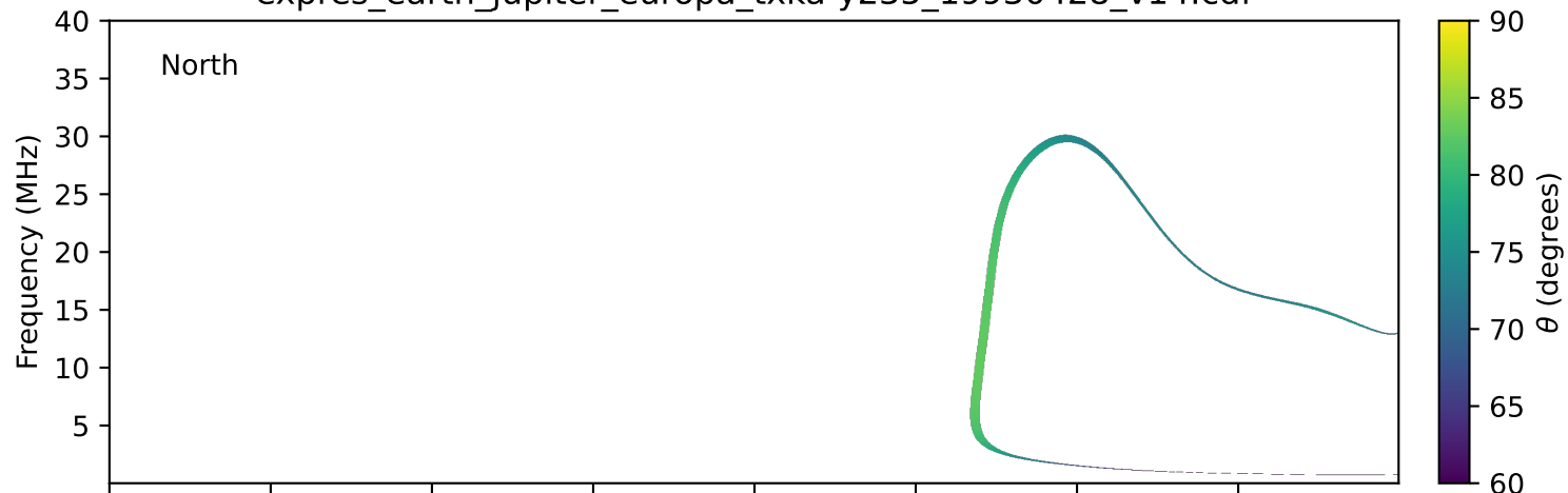
expres_earth_jupiter_europa_txka-y235_19930428_v14.cdf
