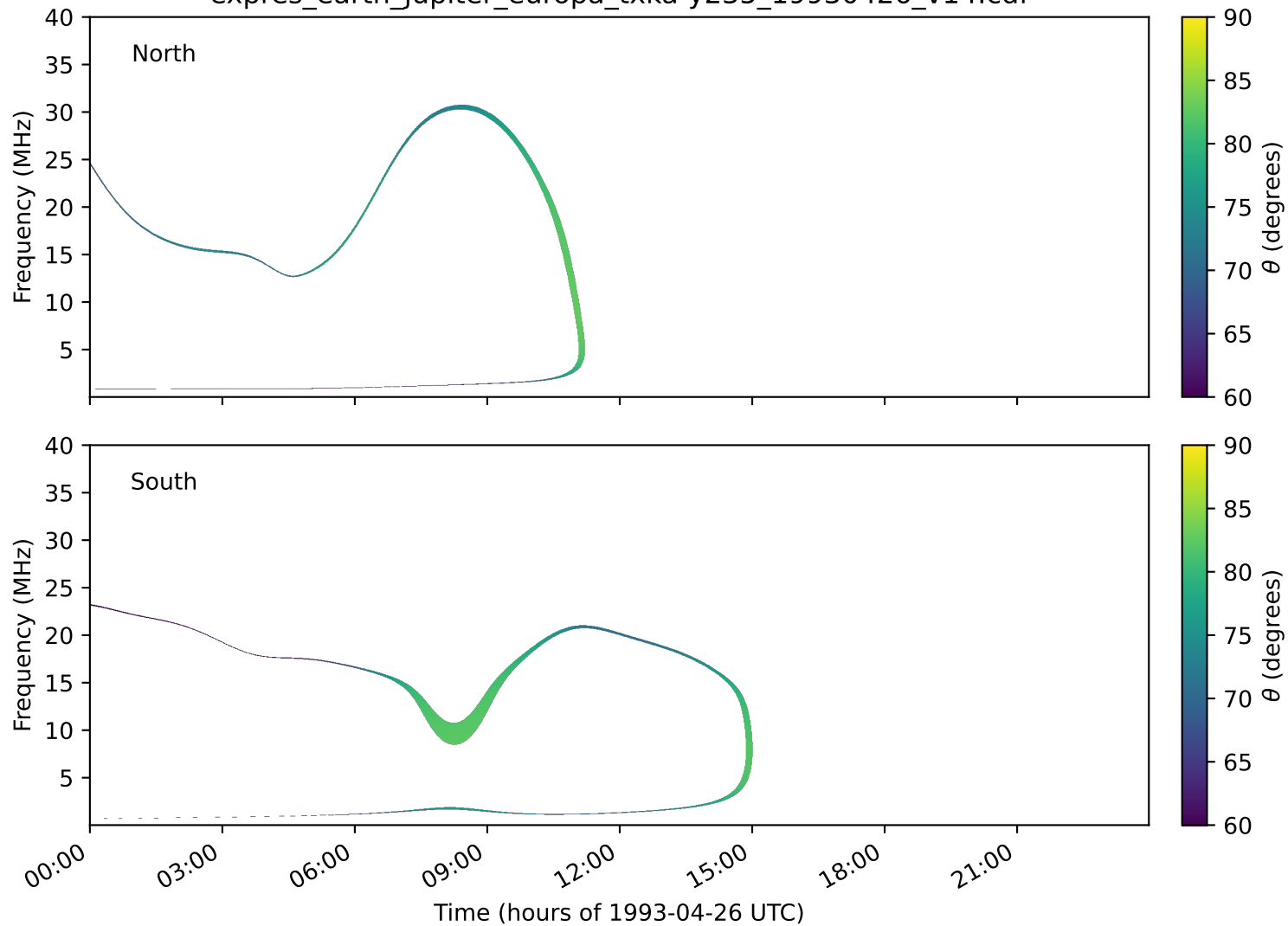
expres_earth_jupiter_europa_txka-y235_19930426_v14.cdf
