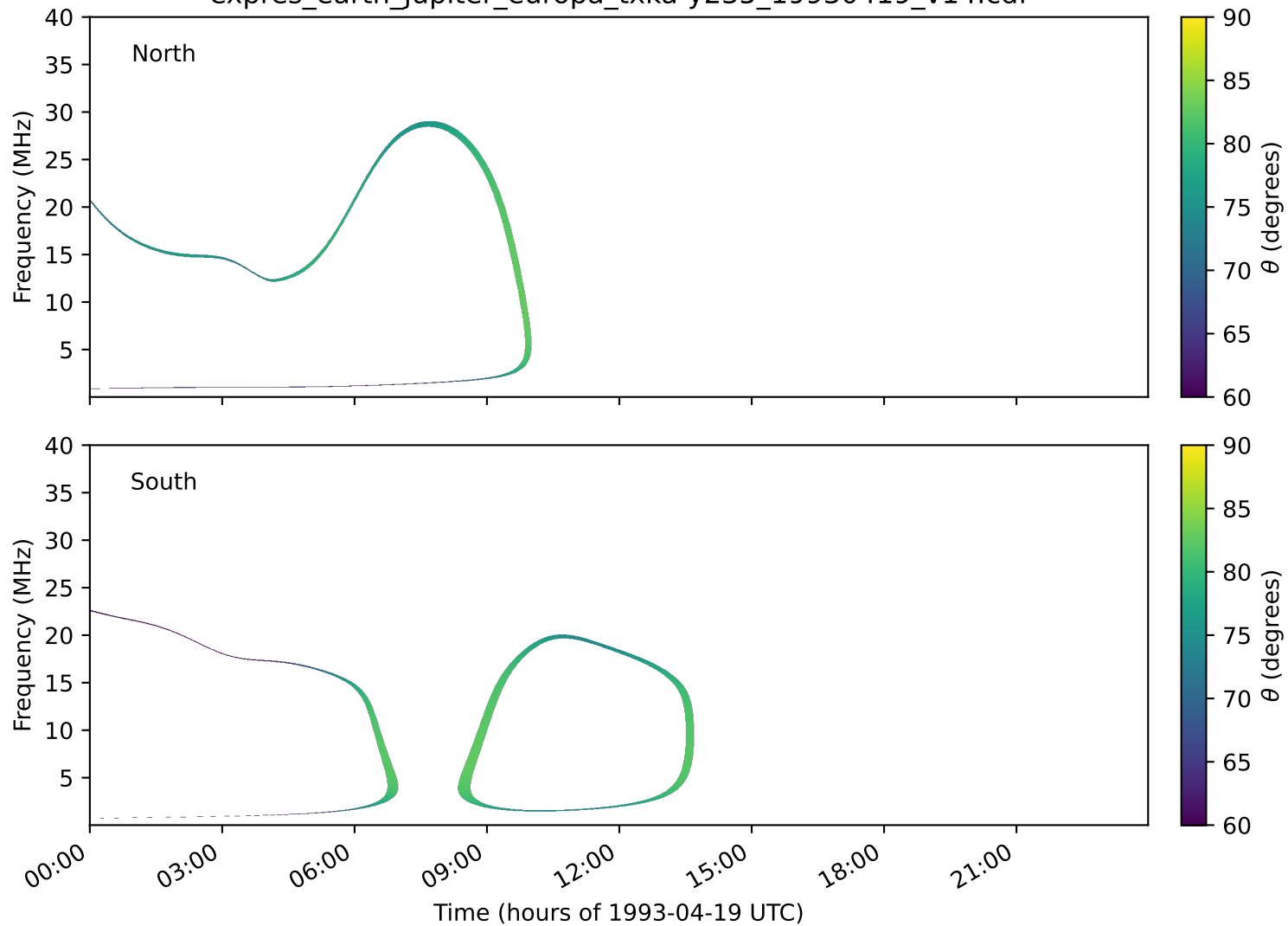
expres_earth_jupiter_europa_txka-y235_19930419_v14.cdf
