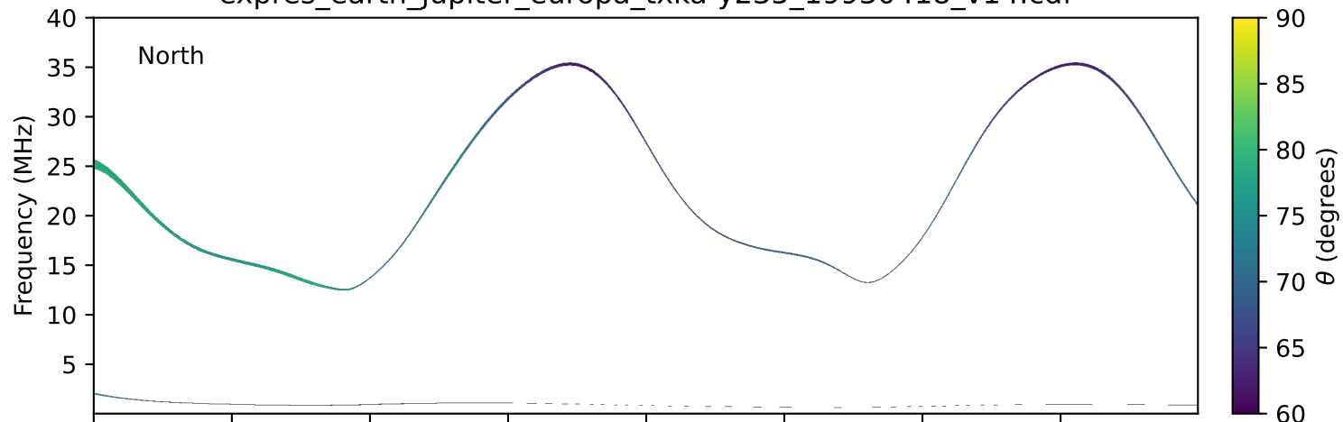
expres_earth_jupiter_europa_txka-y235_19930418_v14.cdf
