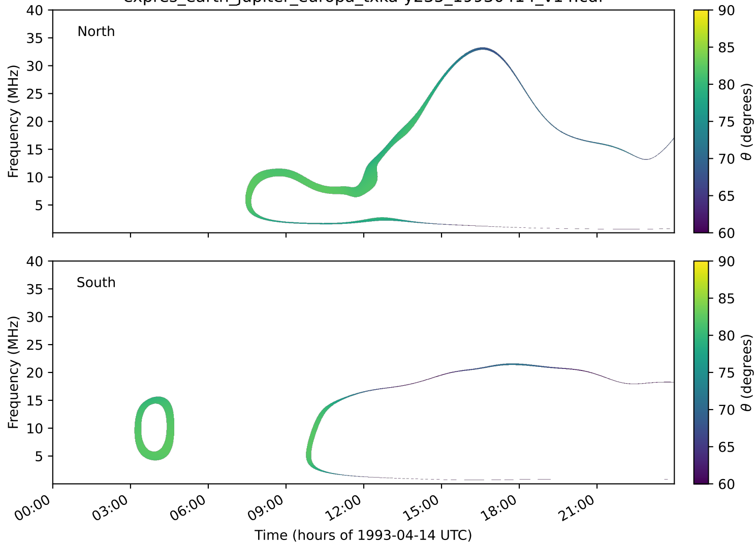
expres_earth_jupiter_europa_txka-y235_19930414_v14.cdf
