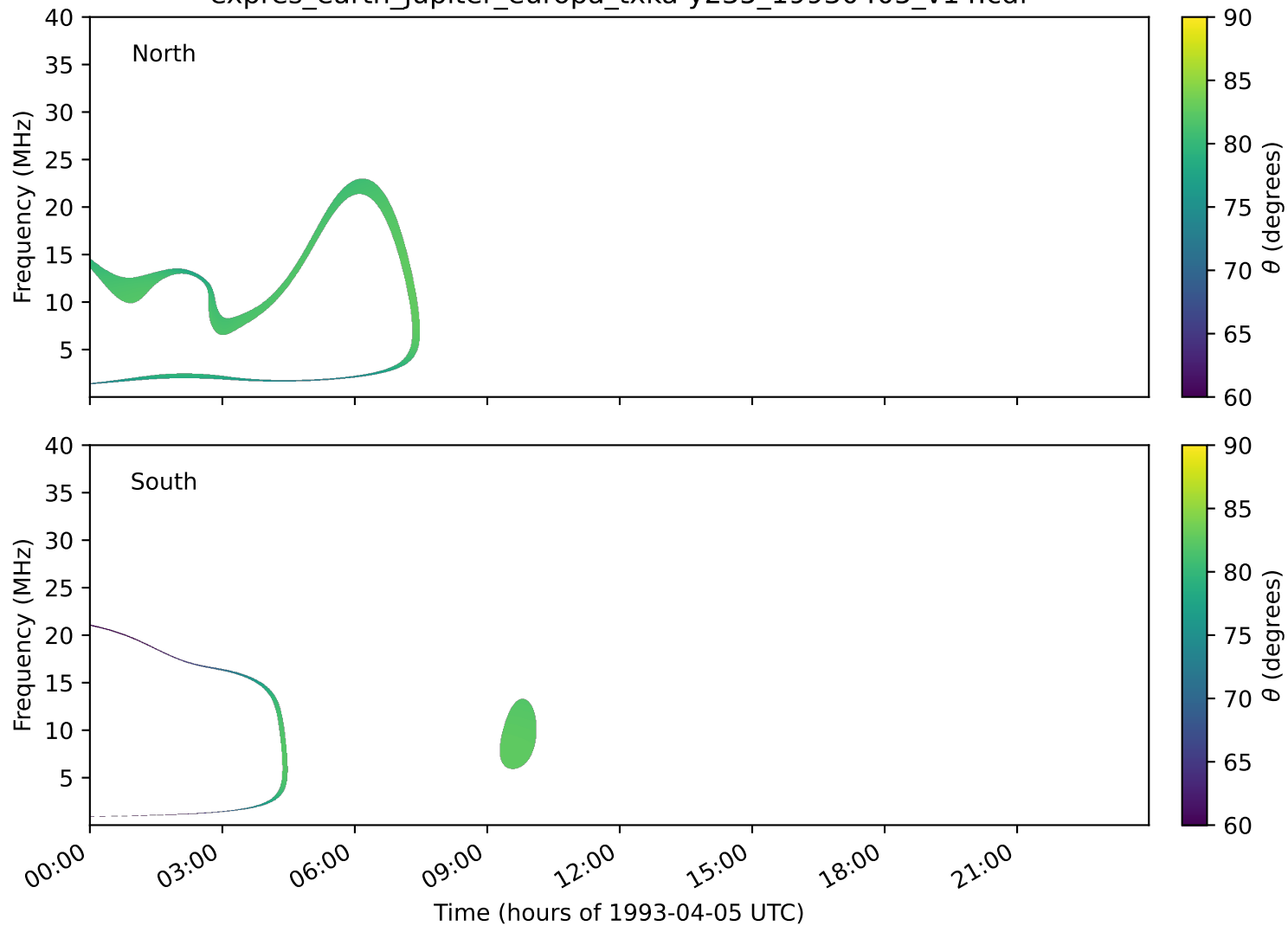
expres_earth_jupiter_europa_txka-y235_19930405_v14.cdf
