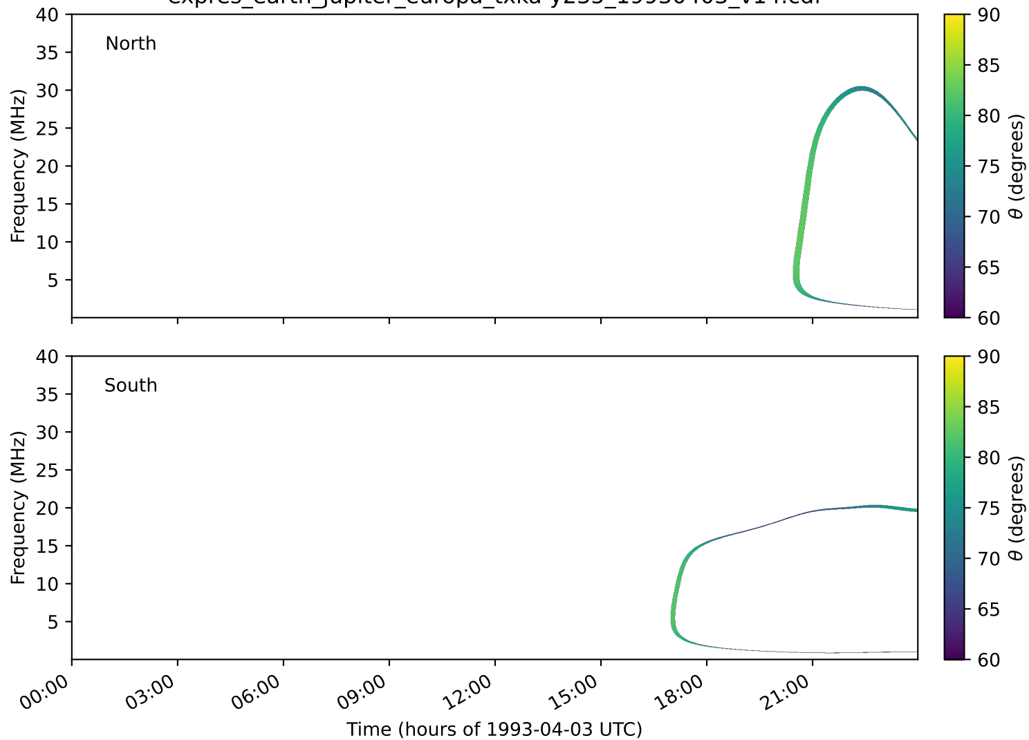
expres_earth_jupiter_europa_txka-y235_19930403_v14.cdf
