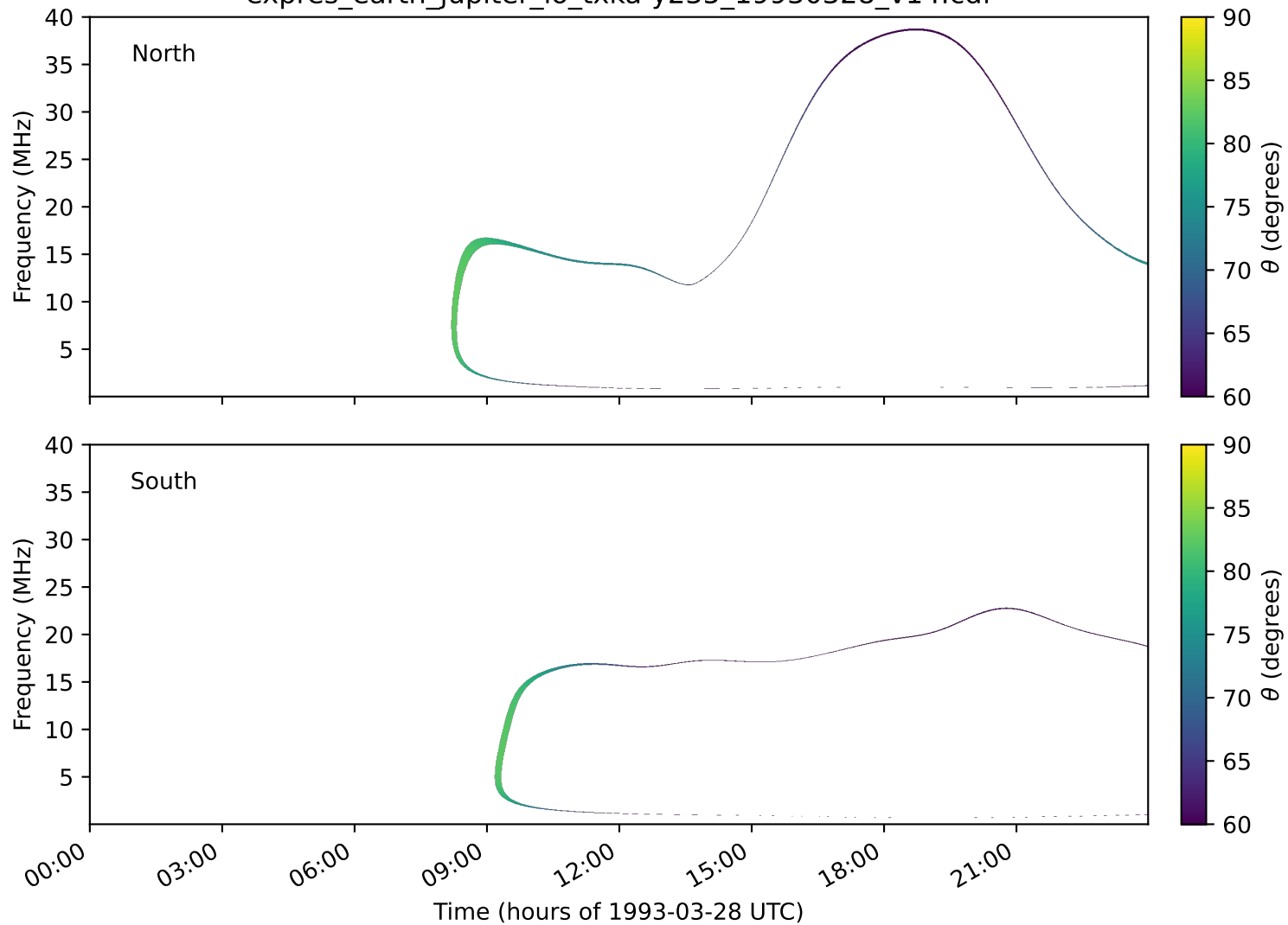
expres_earth_jupiter_io_txka-y235_19930328_v14.cdf
