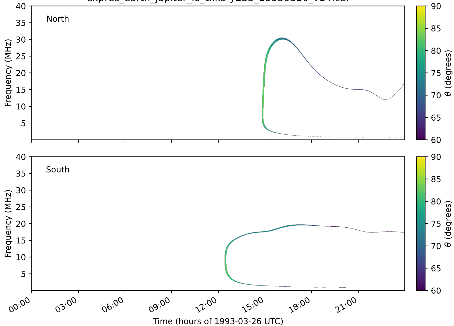
expres_earth_jupiter_io_txka-y235_19930326_v14.cdf
