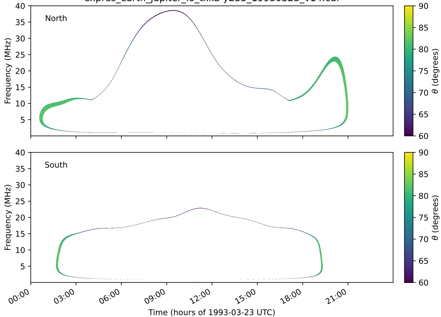
expres_earth_jupiter_io_txka-y235_19930323_v14.cdf
