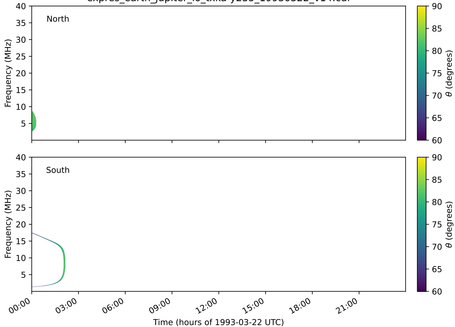
expres_earth_jupiter_io_txka-y235_19930322_v14.cdf
