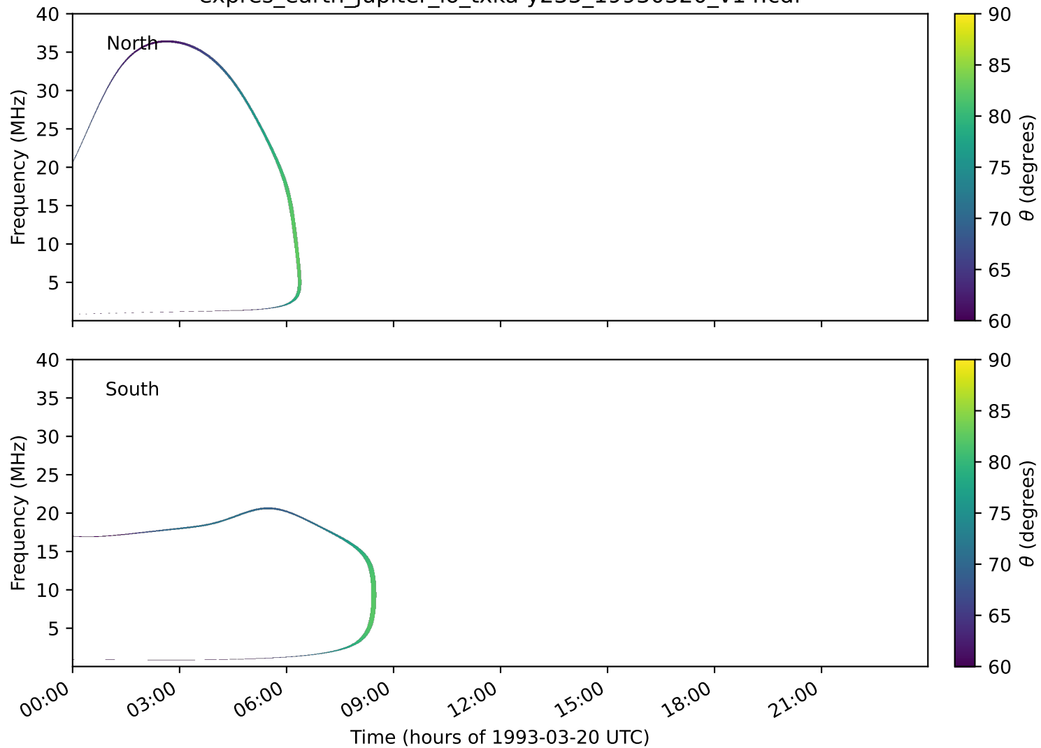
expres_earth_jupiter_io_txka-y235_19930320_v14.cdf
